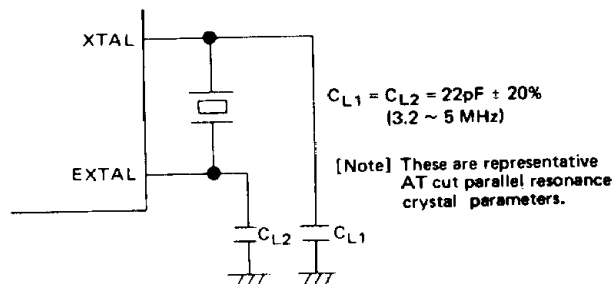
Figure 12 Crystal Interface
