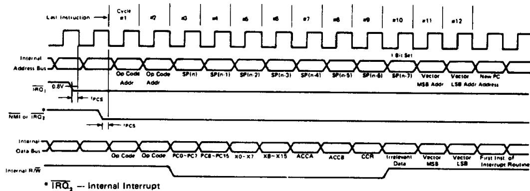
Figure 10 Interrupt Sequence
