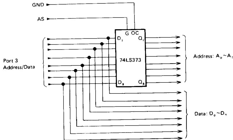
Figure 19 Latch Connection
