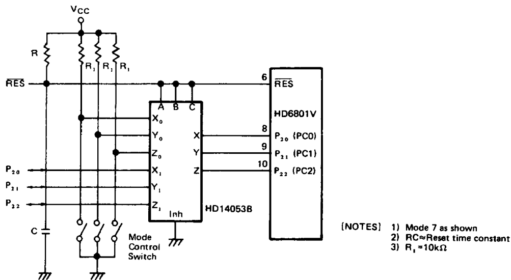
Figure 14 Recommended Circuit for Mode Selection
