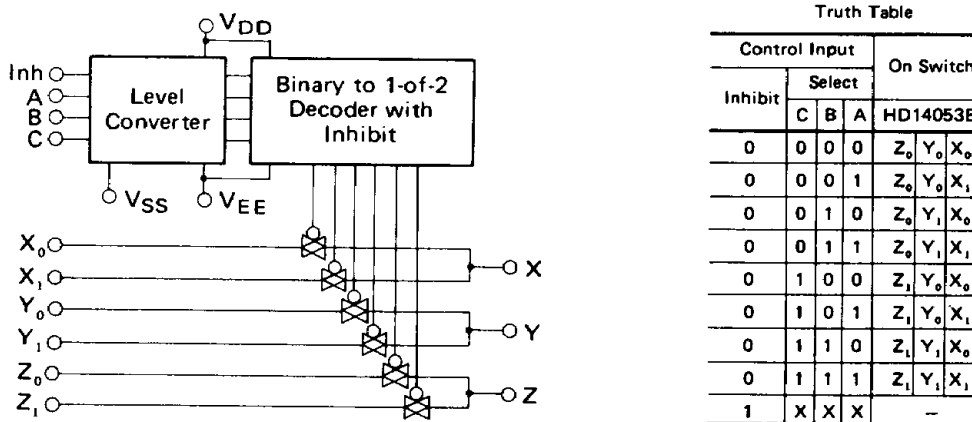
Figure 15 HD14053B Multiplexers/Demultiplexers
