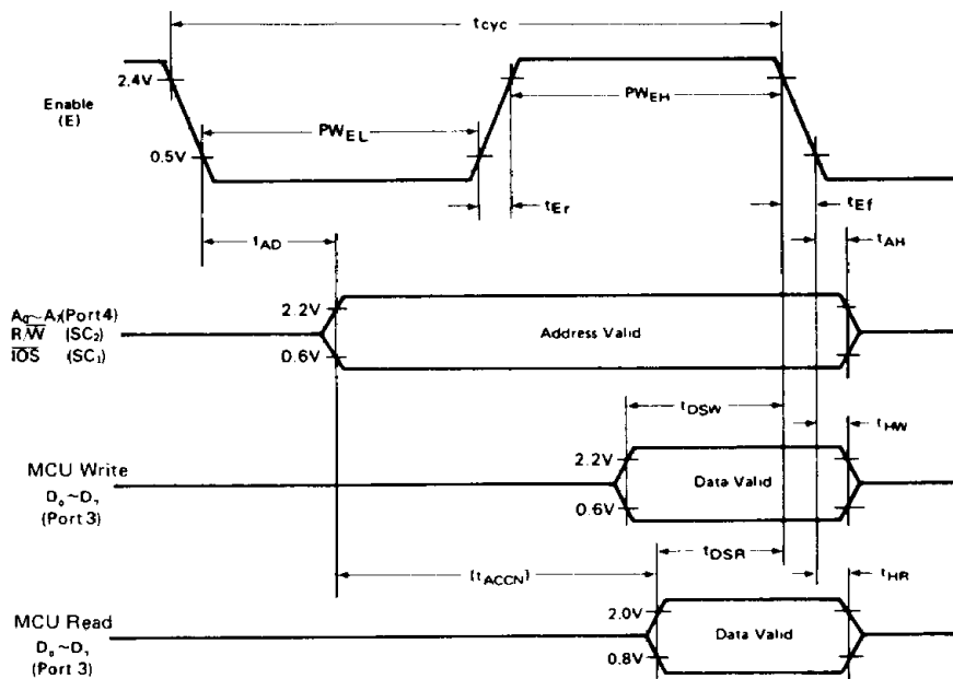
Figure 2 Expanded Non-Multiplexed Bus Timing
