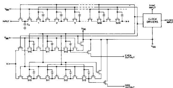
Figure 2. Equivalent Circuit-Diagram of SAD-512D.
