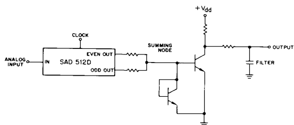
Figure 10. Simple Output Summing Amplifier.
