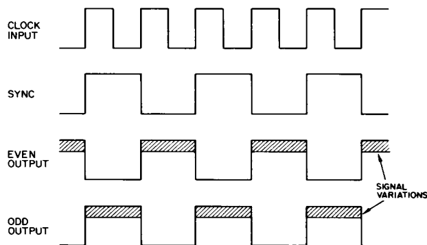
Figure 3. SAD-512D Clock Waveforms.
