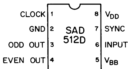
Figure 1. Pin Configuration.
