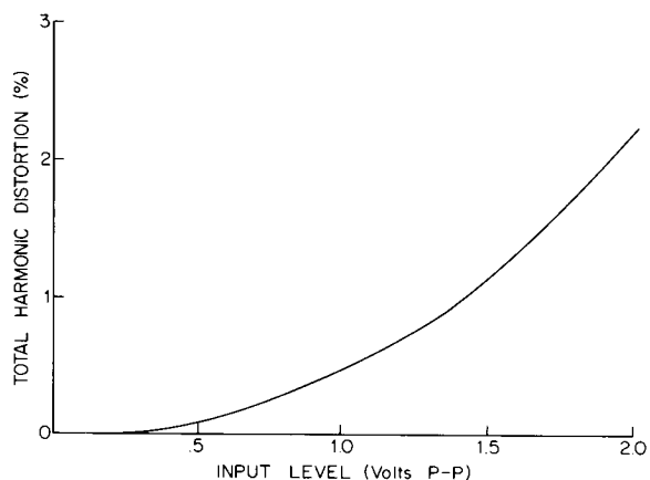
Figure 6. SAD-512D Distortion vs. Input Level.
