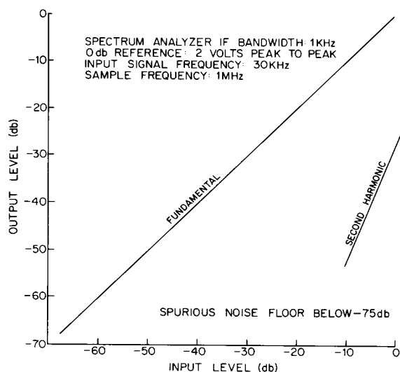
Figure 5. SAD-512D Transfer Characteristic.
